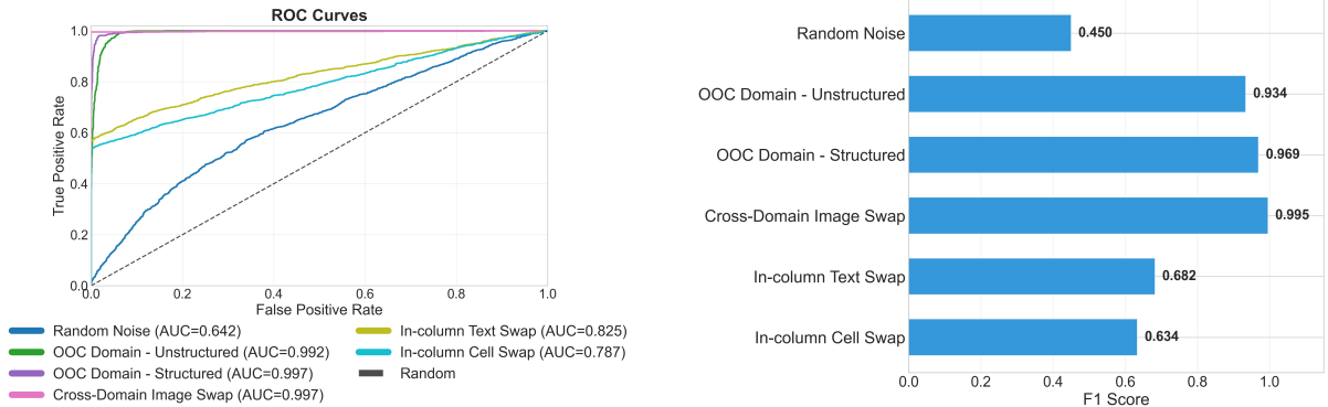
Figure 2: ROC curves (left) and F1@k scores (right) for the Dual-Objective model across six anomaly categories.
